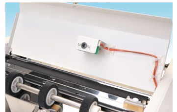
The double feed detection sensor prevents mis-folded papers being contaminated to outputs.
